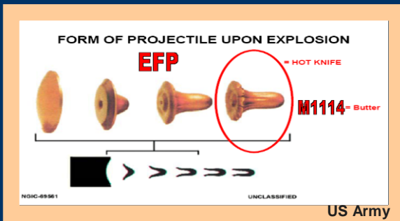
Figure 2. An Explosively Formed Penetrator
